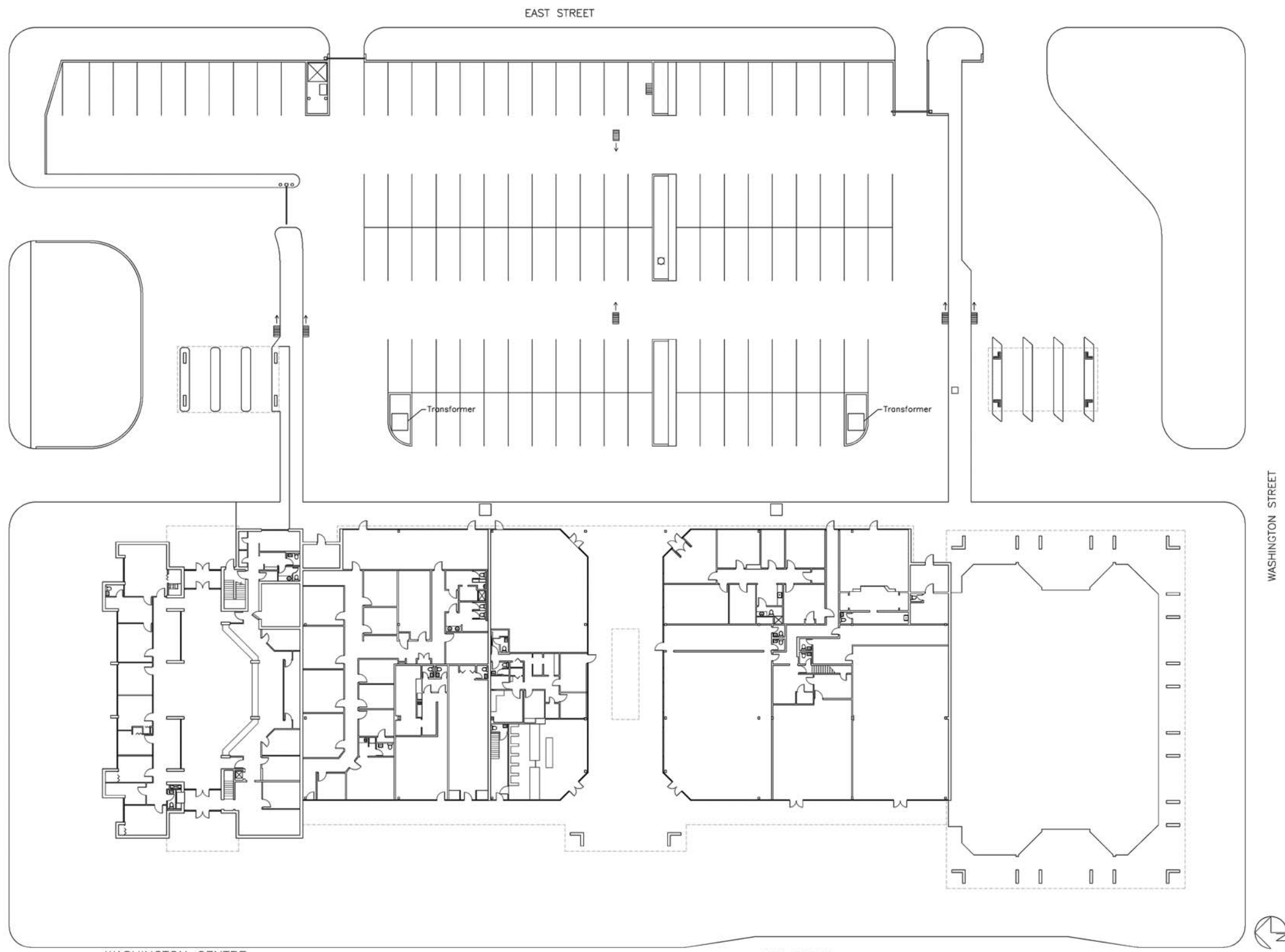
WASHINGTON CENTRE Scale: 1"=40'-0"
